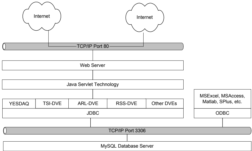
Figure 6. Component Architecture
